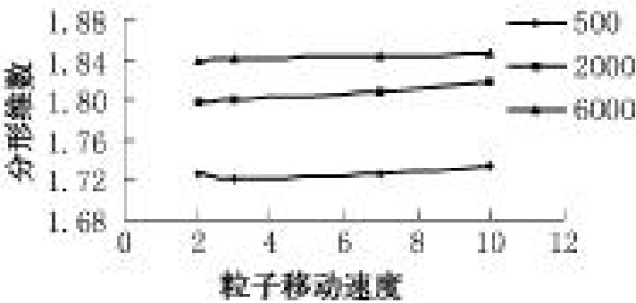
图6 粒子移动速度对沉积产物分形维数关系曲线 Fig.6 The relation curve about particle migration rate vs. fractal dimension of electrodeposition
